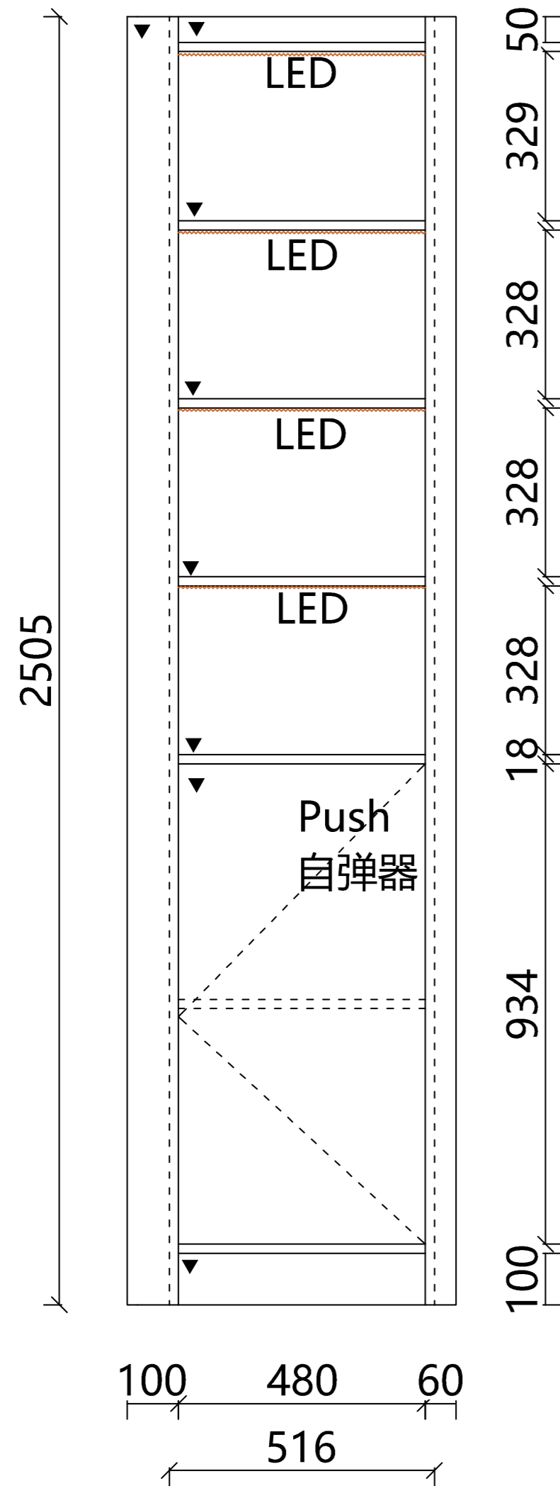
ELEVATION C
