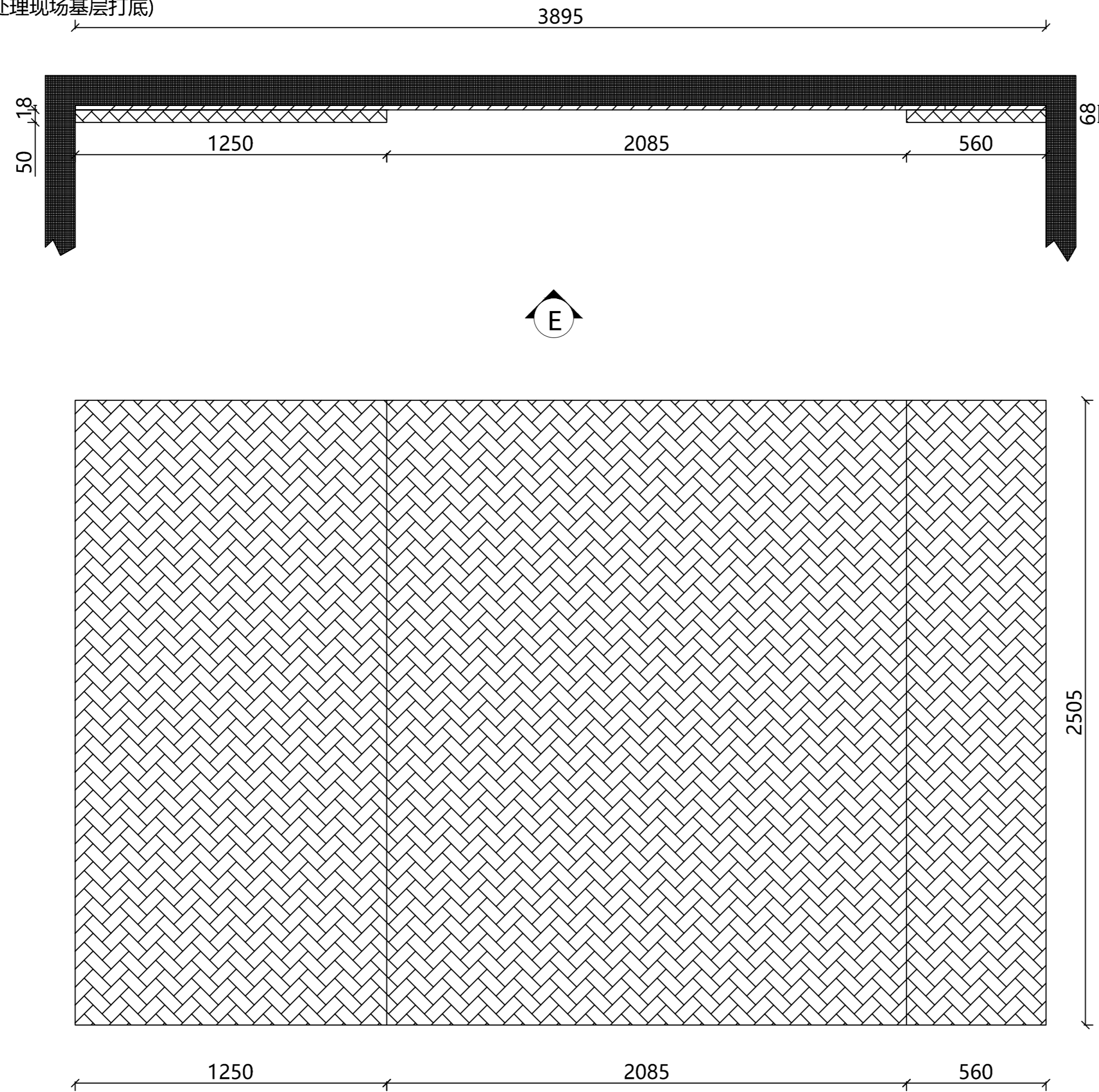
STRUCTURE E
