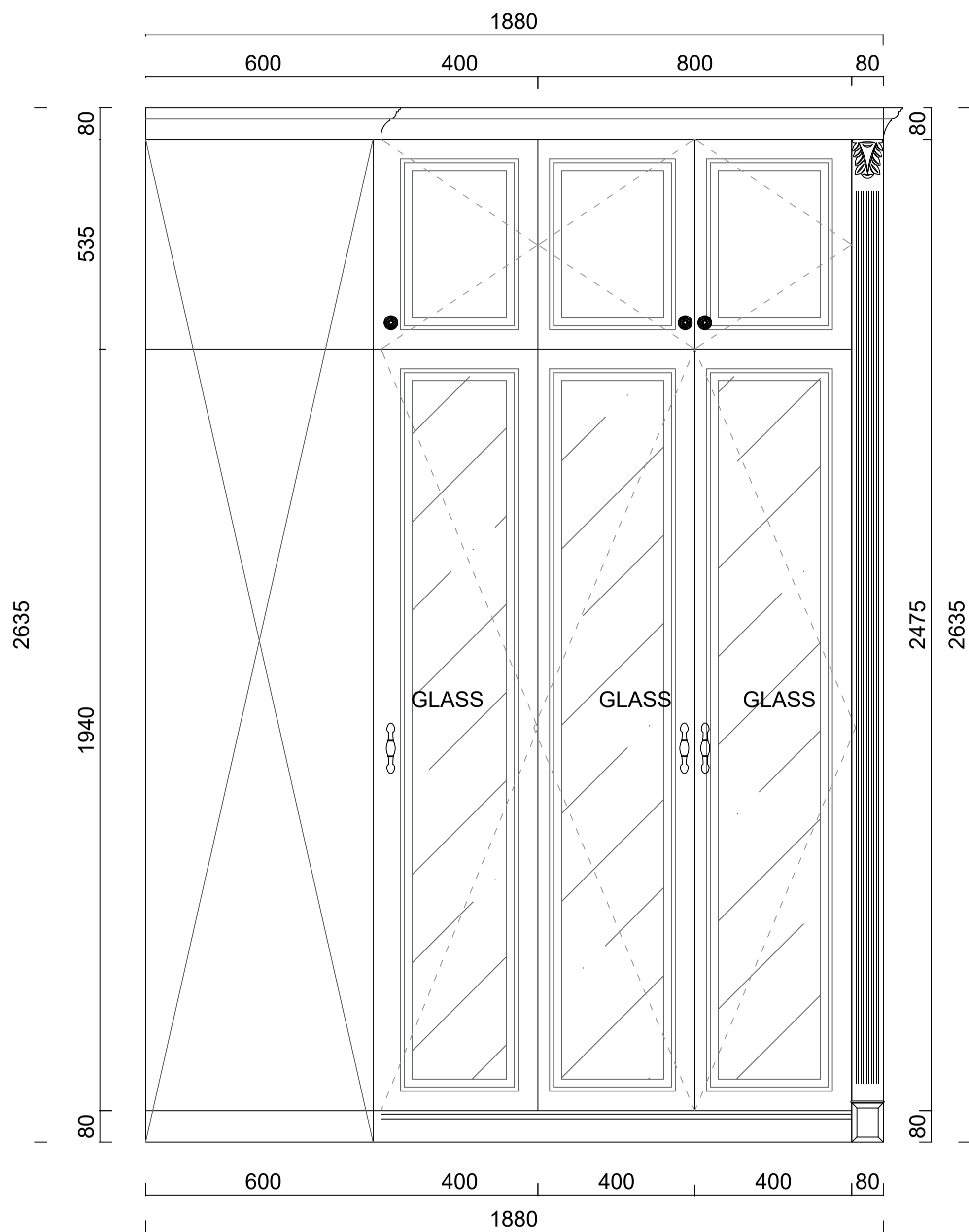
D ELEVATION
