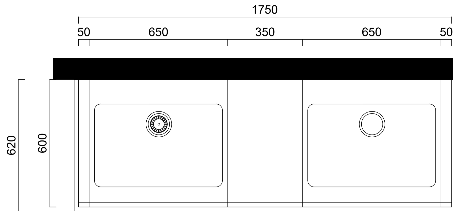
PLAN
