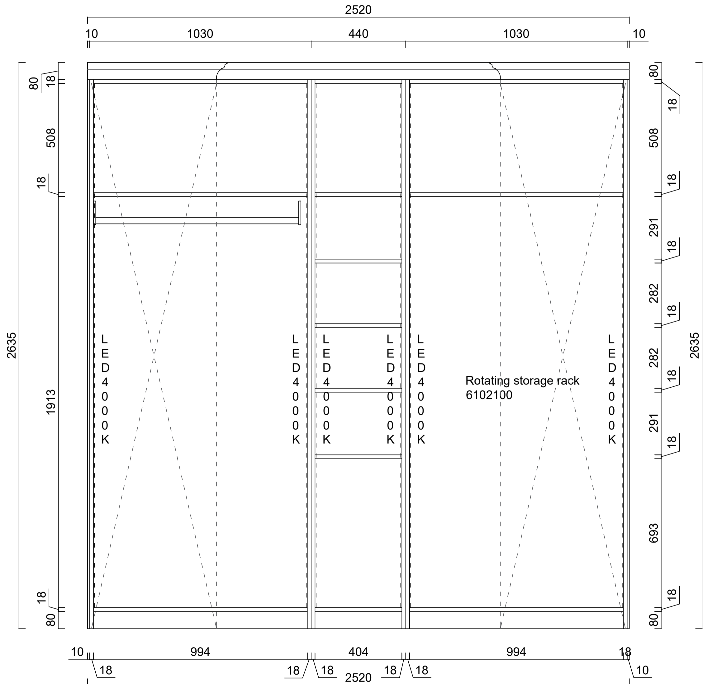
B STRUCTURE
