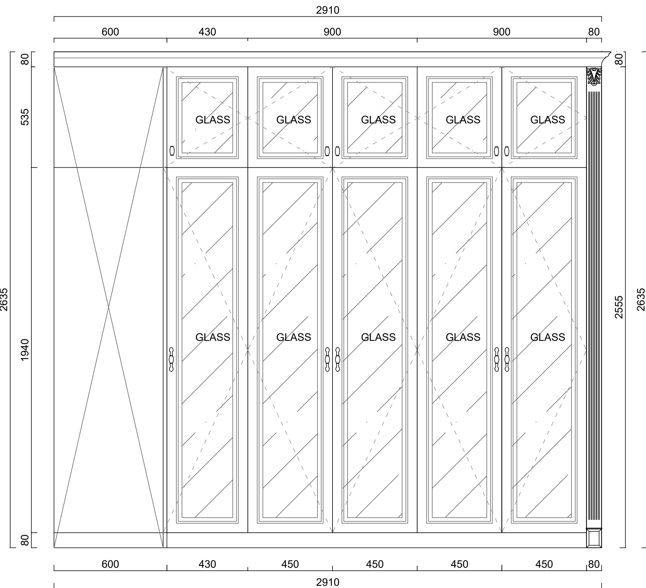
C ELEVATION
