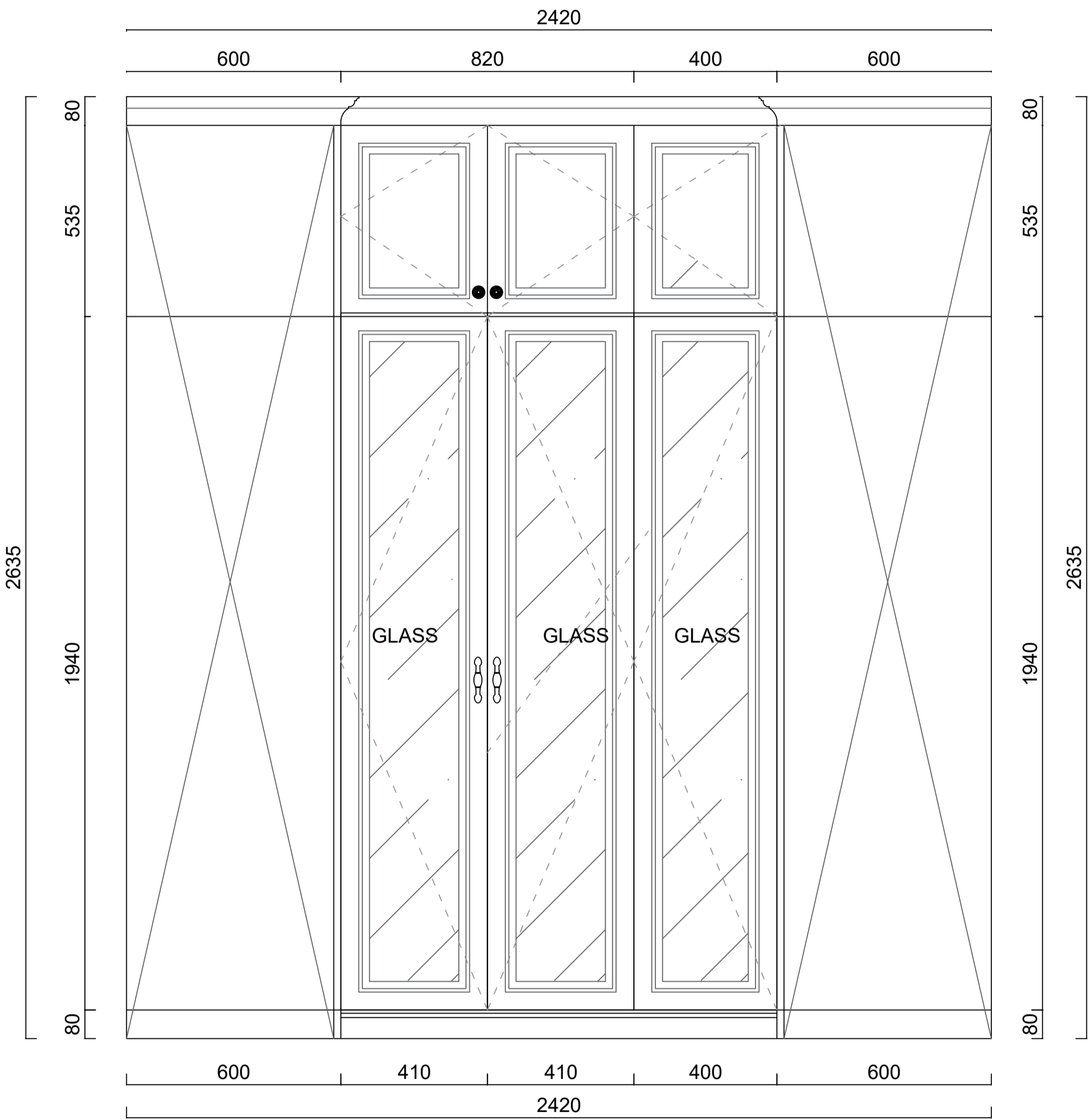
C ELEVATION
