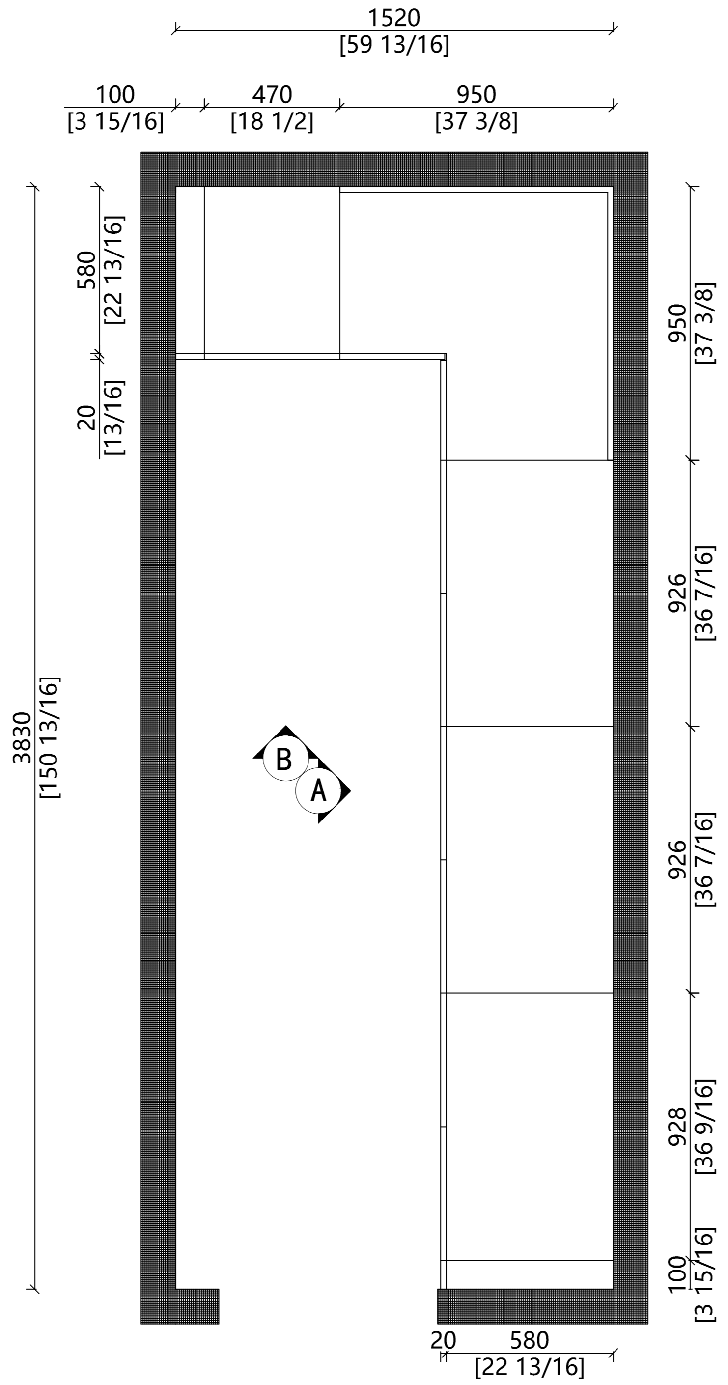
Plan
