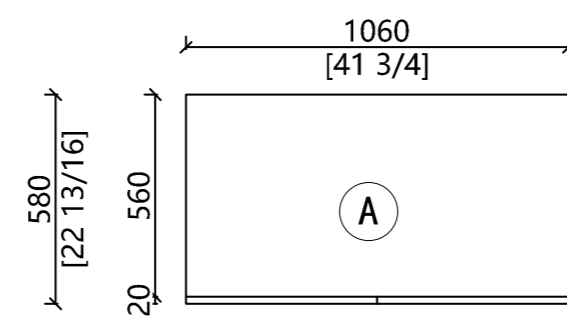
Plan A
