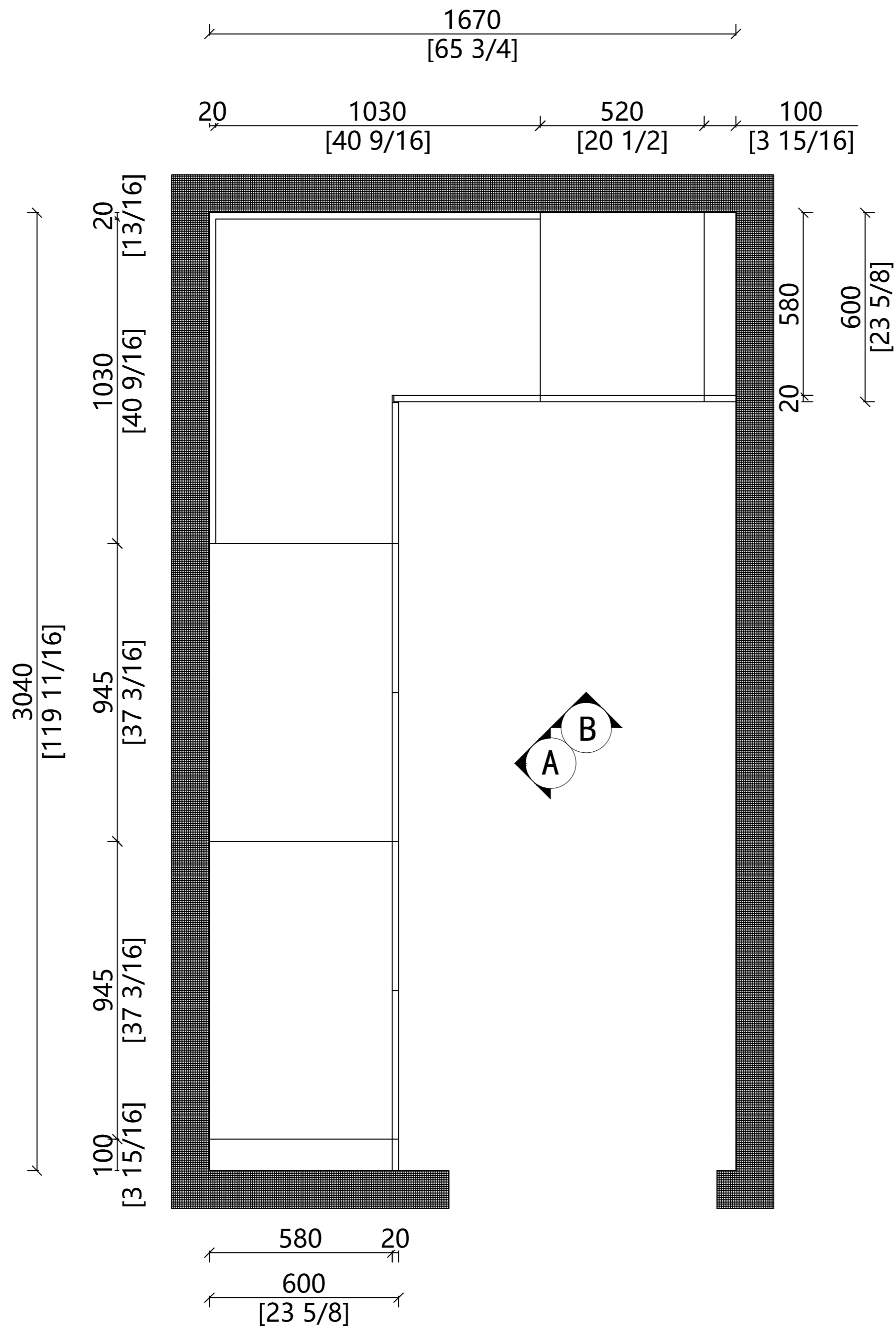
Plan
