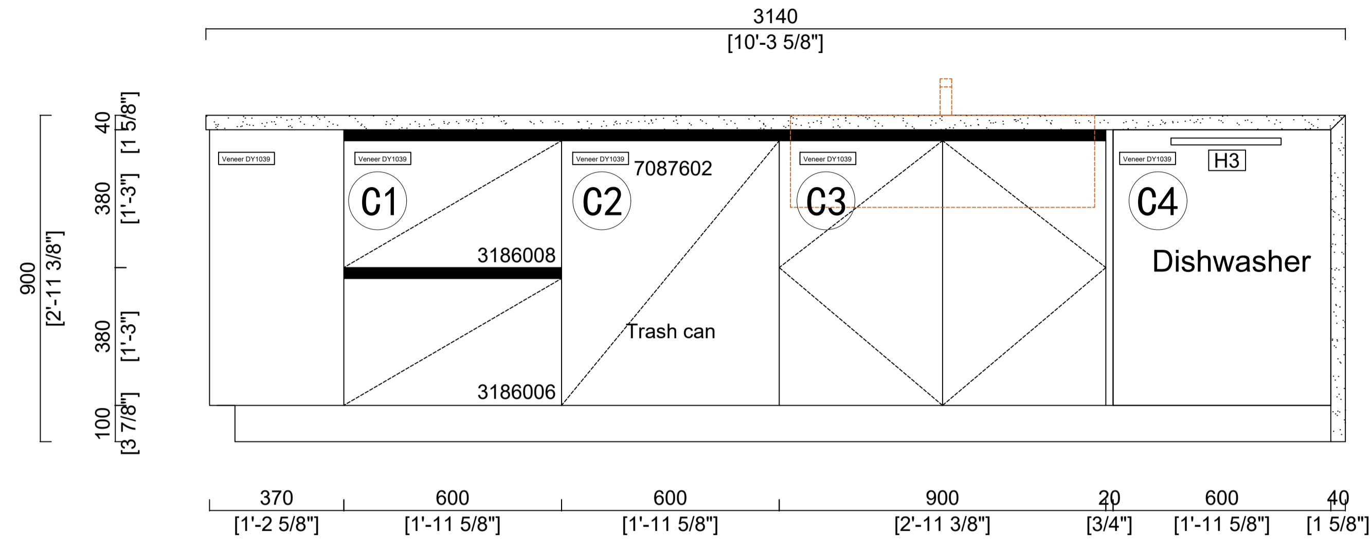
ELEVATION C
