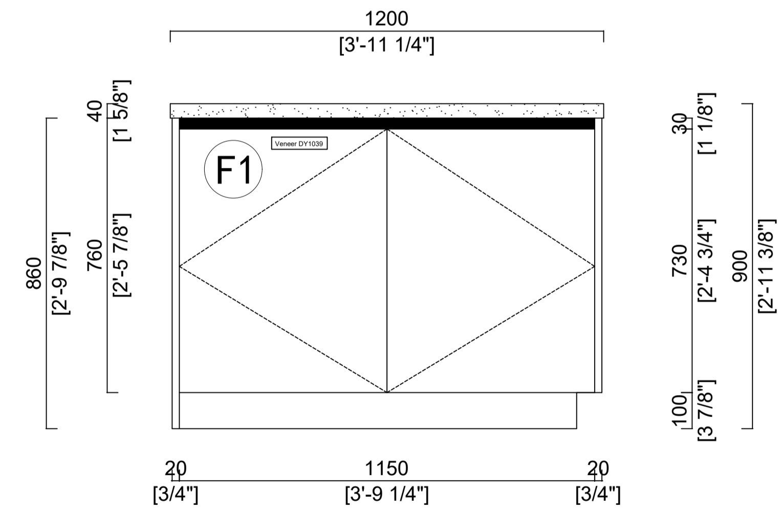
ELEVATION F
