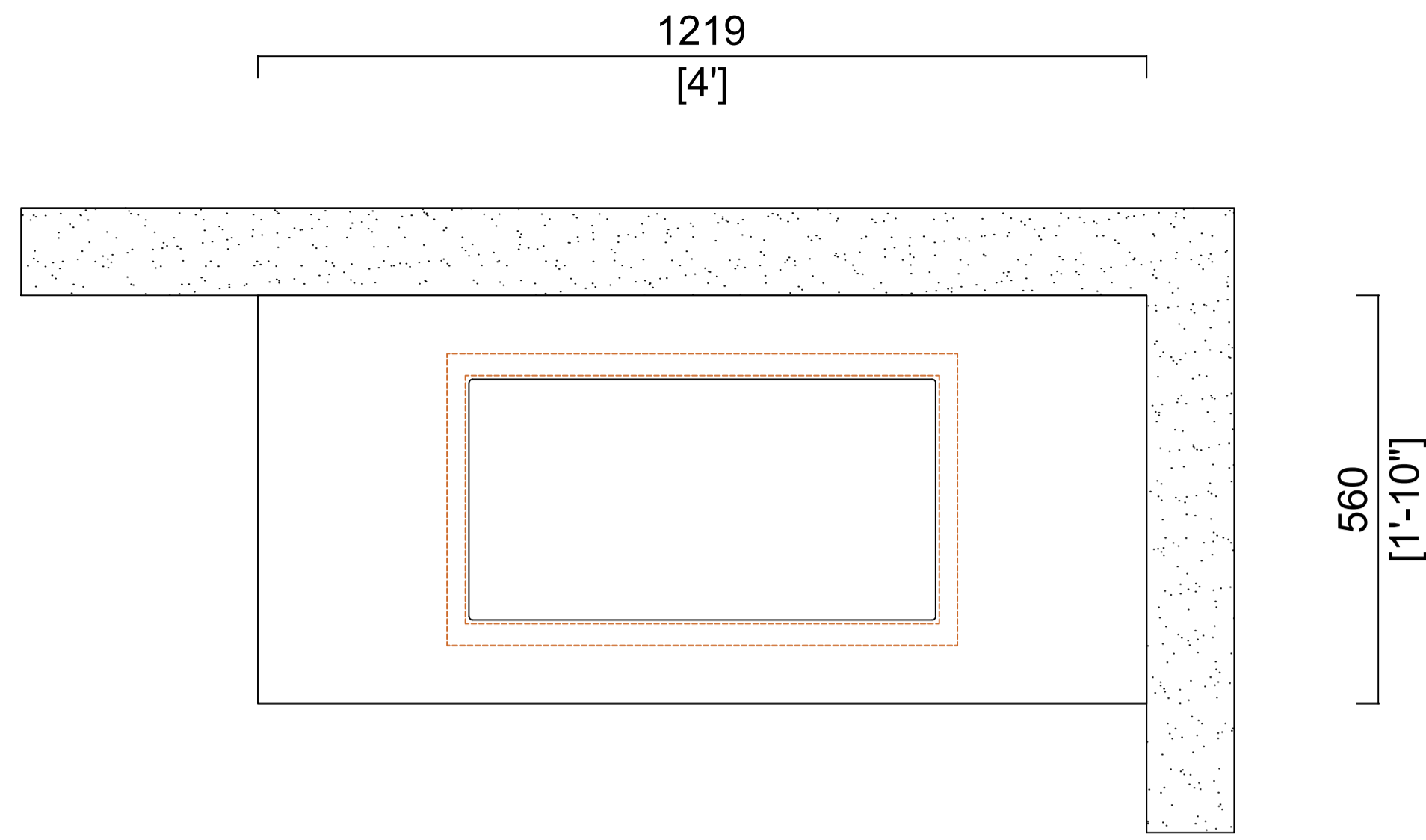
PLAN
